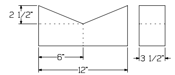
WOOD BUNK FOR 4-TBR80
