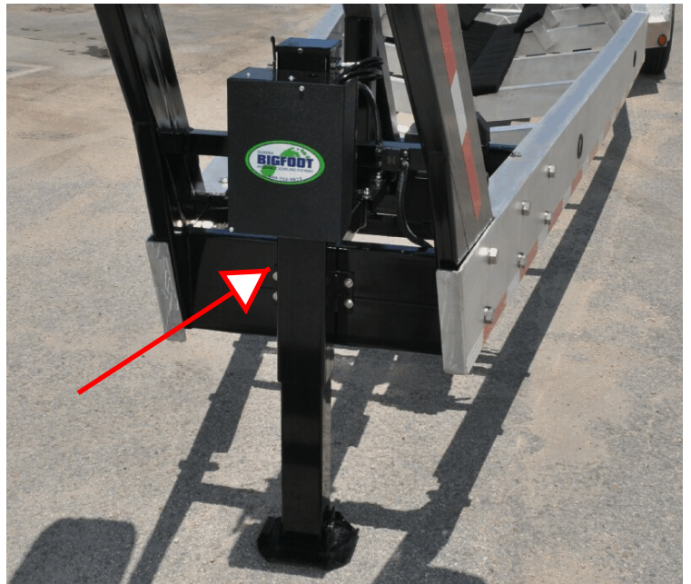
Electro/Hydraulic Jack with battery
